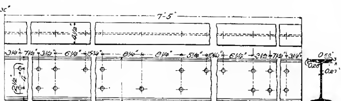
Figs. 4664-4666. Bolster I-Beam, Steel (2).
